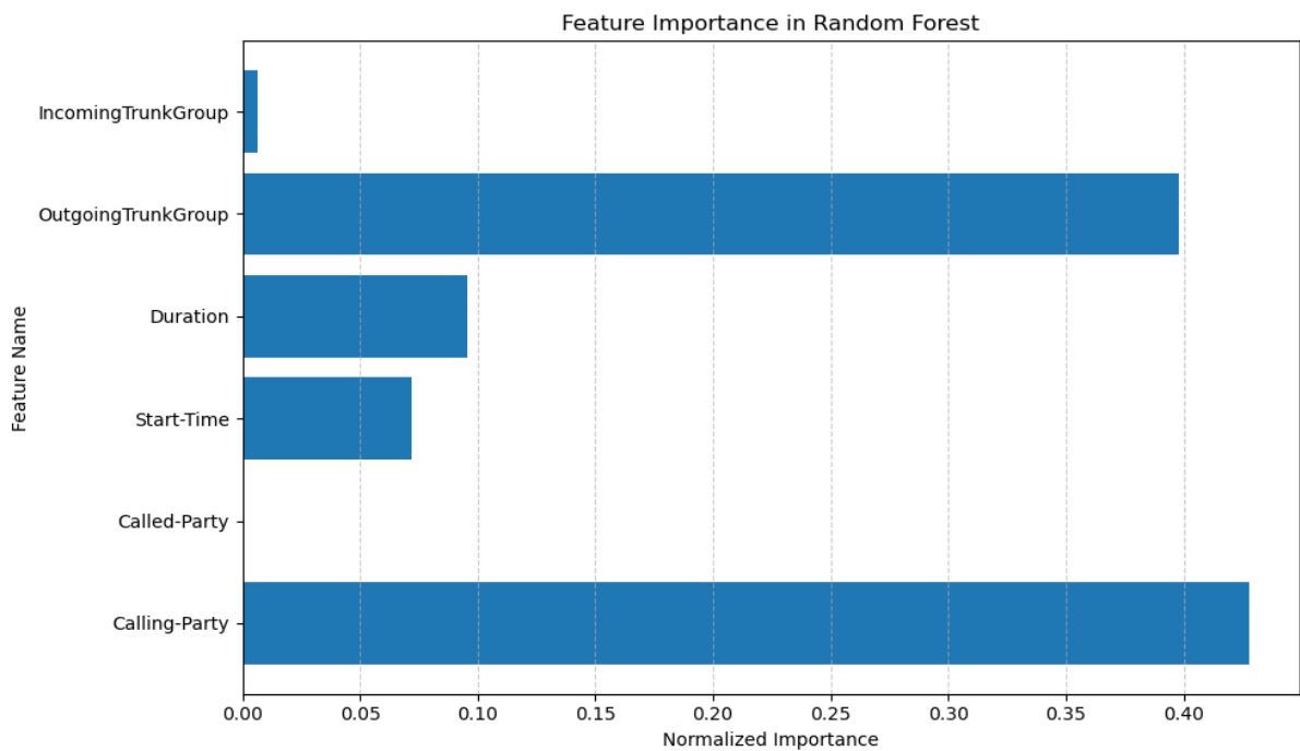
Figure 3. Feature Importance in Random Forest
