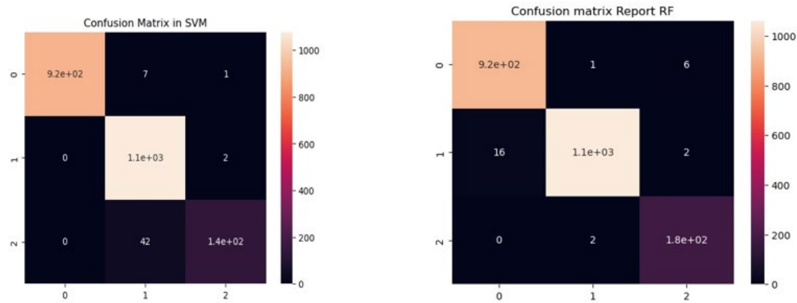
Figure 4. Confusion matrix for SVM and Random forest
