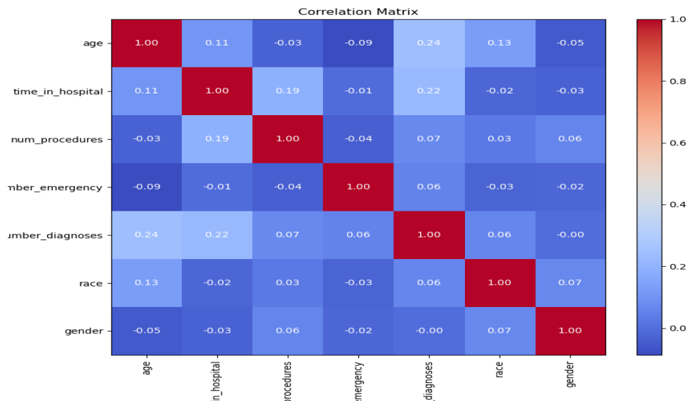
Figure 2. Correlation Matrix
