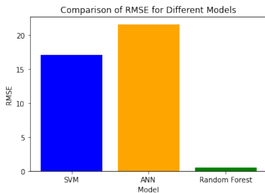
Figure 6. Region 3 RMSE computations. The RF had the lowest value of 0.5054.
