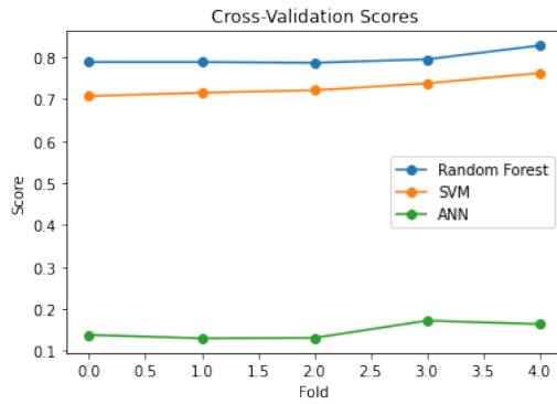
Figure 4. Region 1 Cross-validation scores. The RF had the highest values across all folds.
