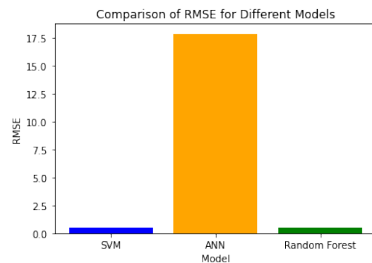
Figure 3. Region 2 RMSE computations. The RF had the lowest value of 0.51.
